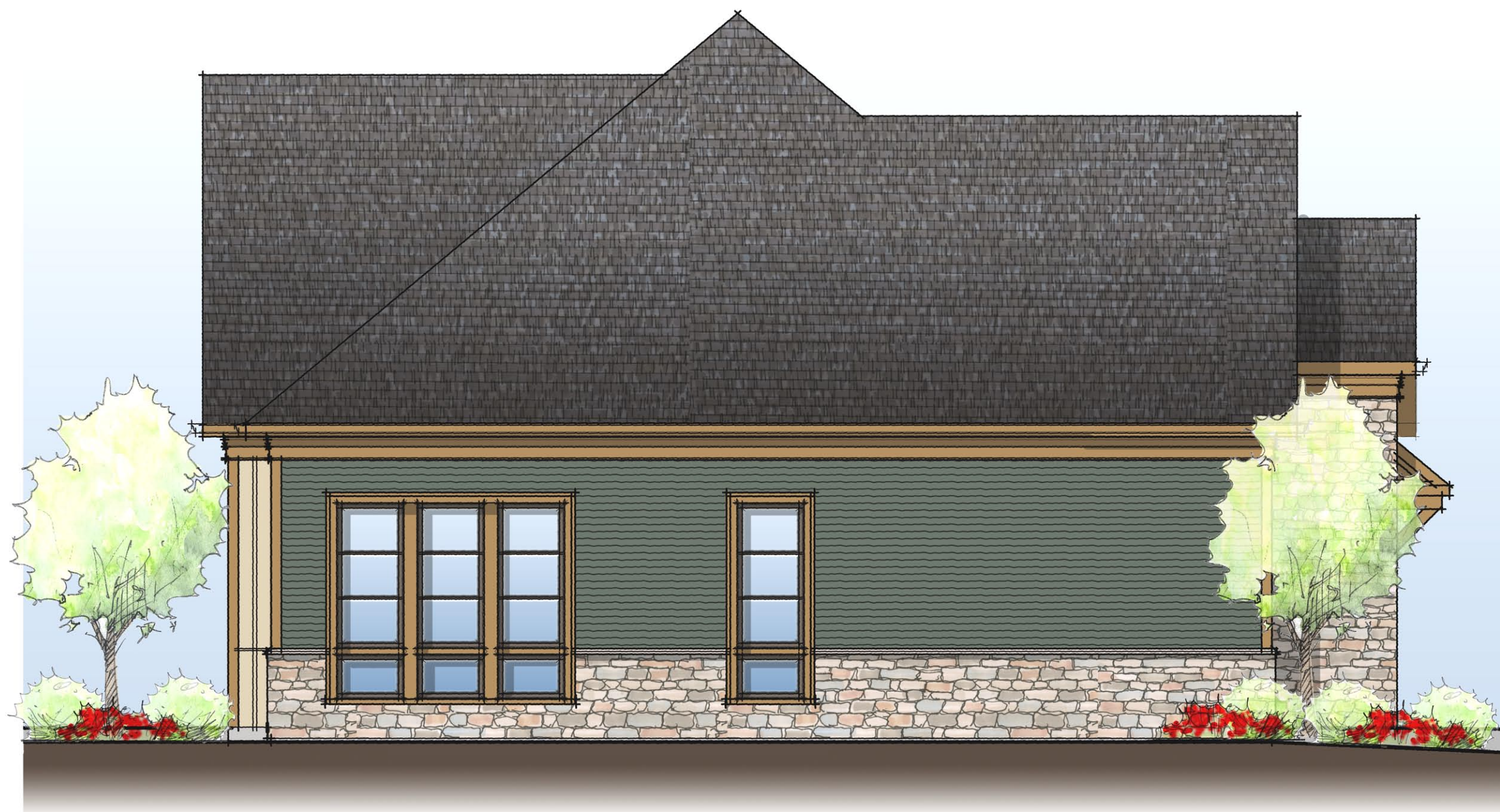
Left Elevation
